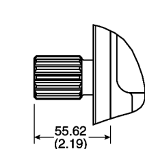
轴伸选项 "B" SAE "C" 花键 14 齿 12/24 径节 最大转矩 = 639 N·m (5,680 IN-LBS)
