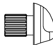
轴伸选项 "D" SAE "C-C" 花键 17 齿 12/24 径节 最大转矩 = 1,218 N·m (10,780 IN-LBS)
